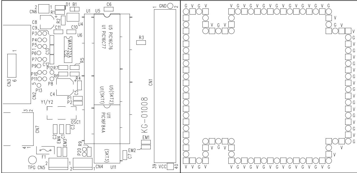
L1 SILK
