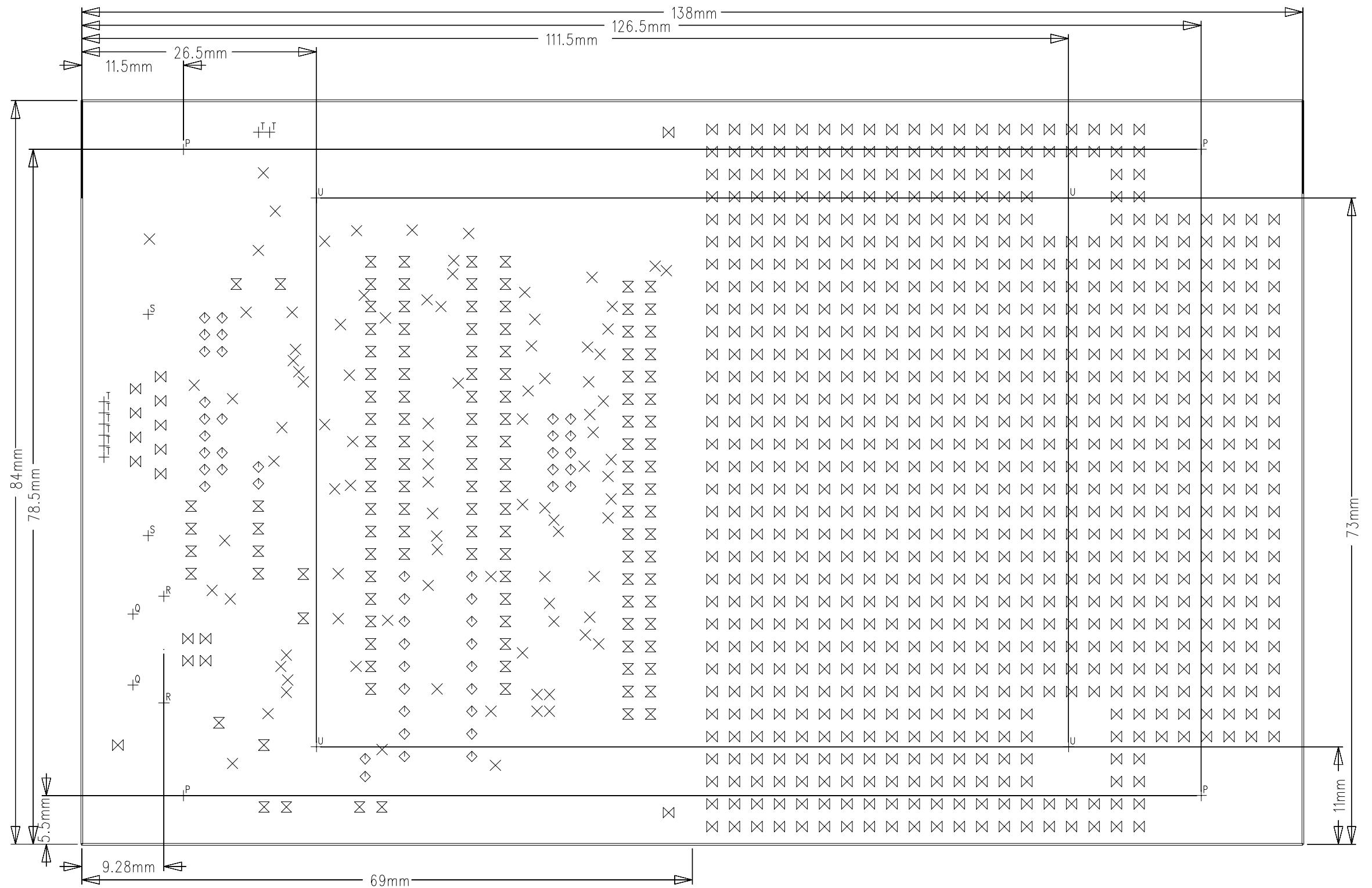
KG-02003A CPU(PIC/USB/RS232C) BOARD DRILL HOLE
